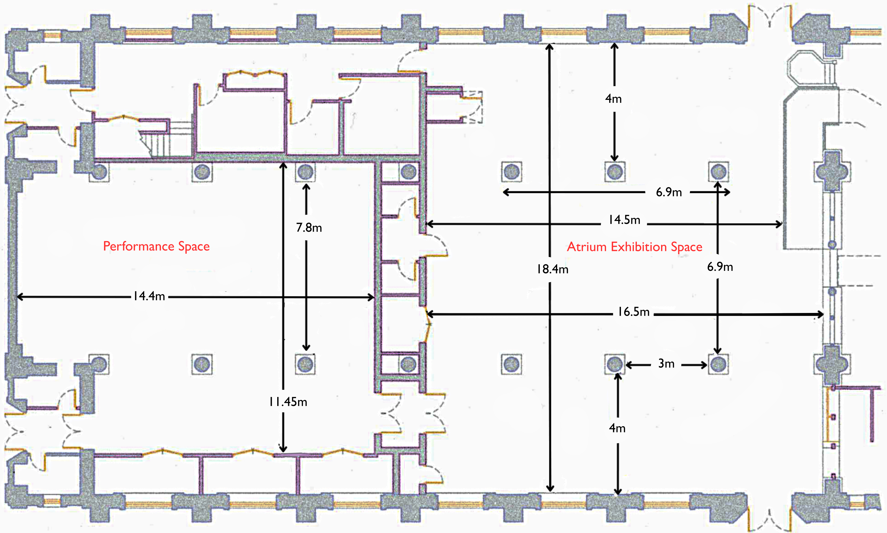
The Horton - Ground Floor Plan
